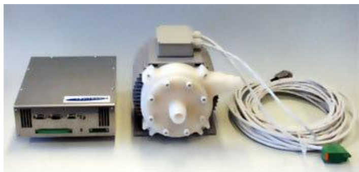
Figure 2: Bearingless pump system for AC voltage supply BPS-4
