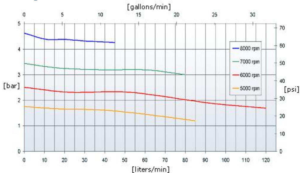
Figure 12: Pressure-flow curves for BSP-4 with water @ 25°C
