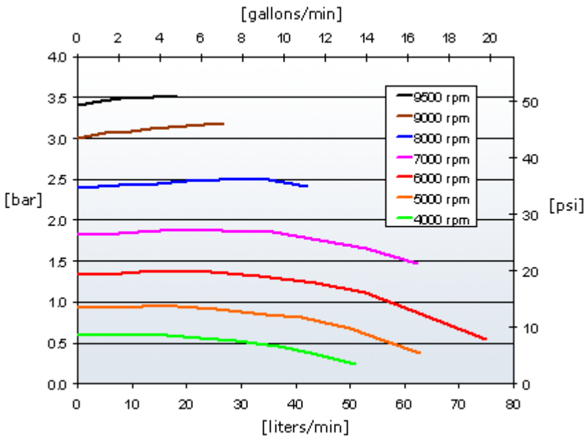
Figure 8: Pressure-flow curves for BSP-3 with water @ 40°C
